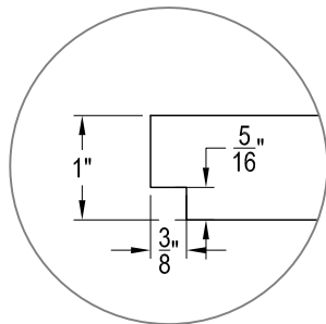
TYP. END DETAIL FOR ALL PANELS
