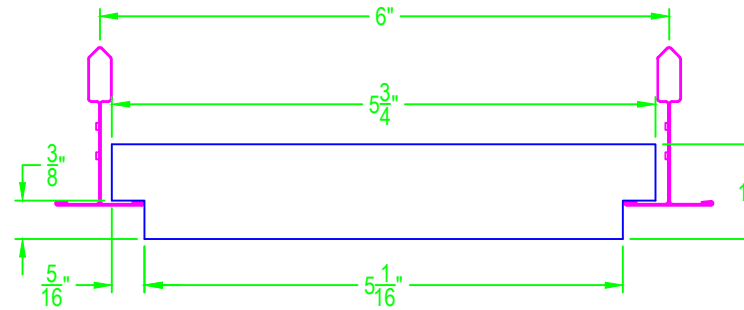
CROSS SECTION
