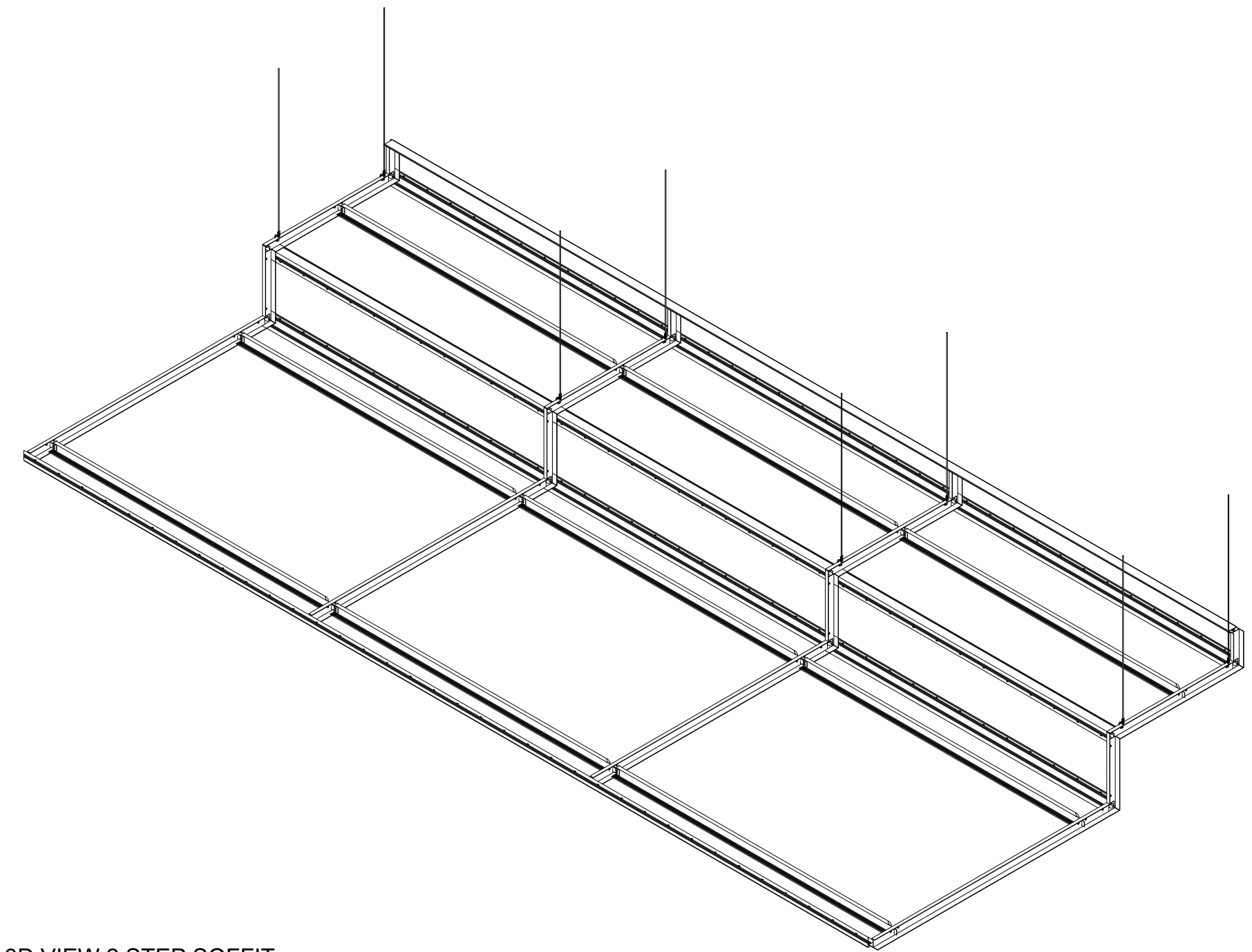
3D VIEW 2 STEP SOFFIT
