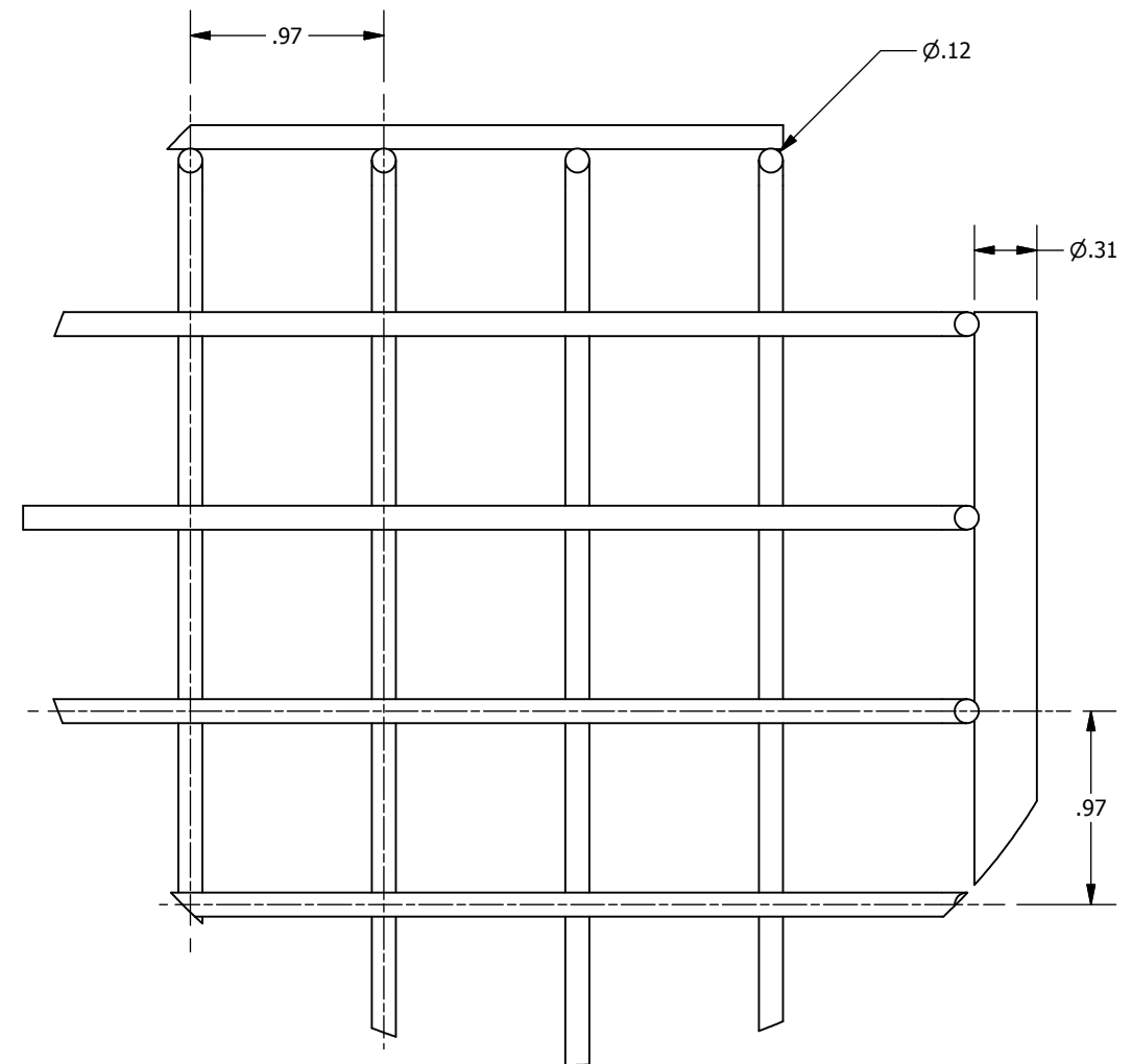
DETAIL A SCALE 1 : 1
