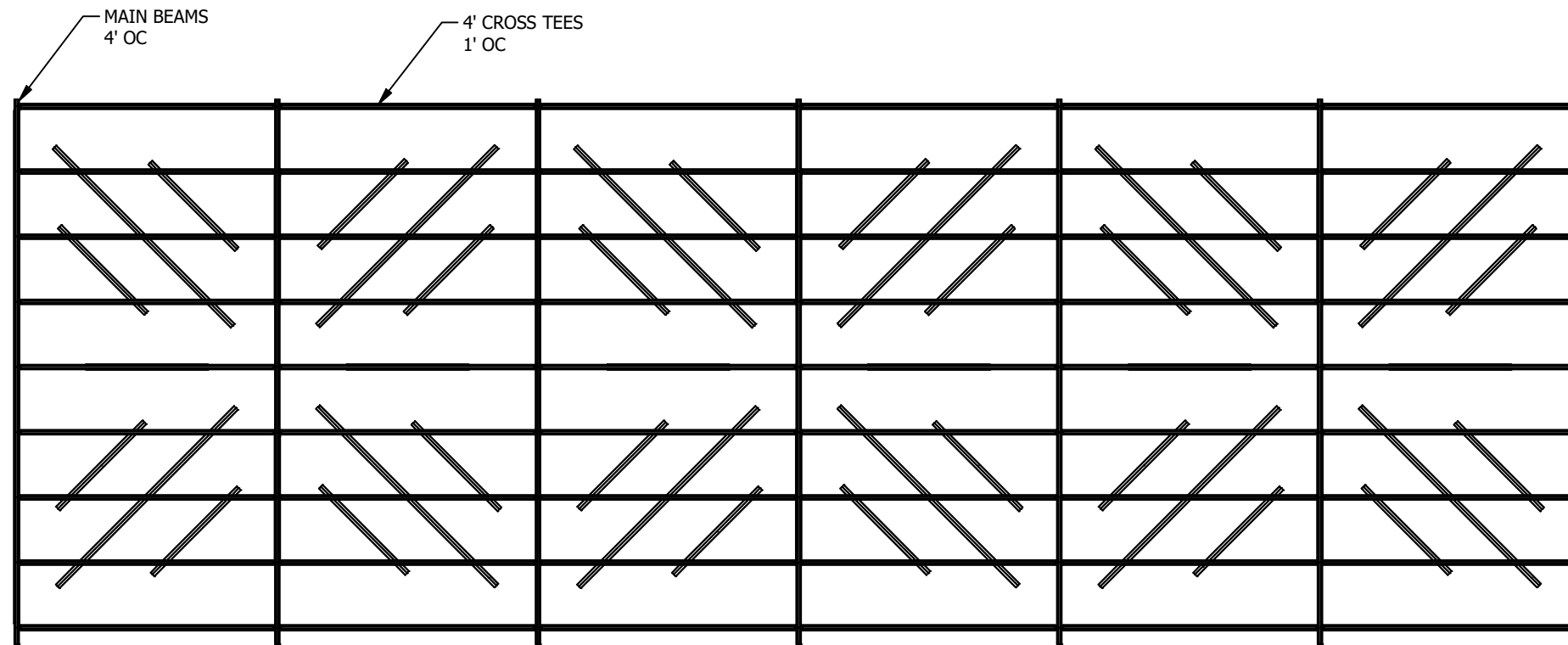
PLAN VIEW
