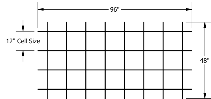
BP6532KOR12R8 R8 12in Rectangular Open Cell Kit
