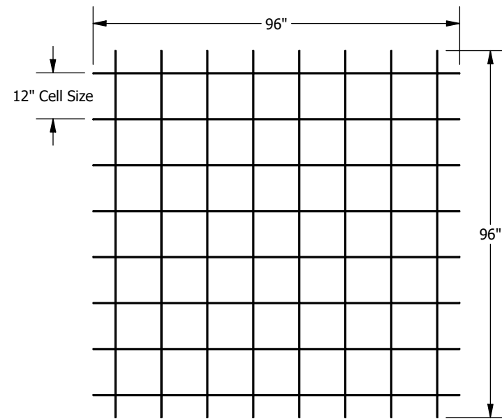
BP6532KOR12S8 S8 12in Rectangular Open Cell Kit
