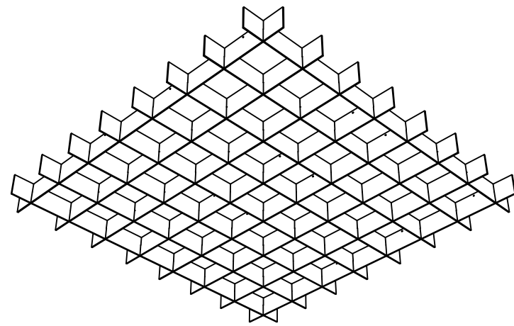
BP6532KOR06S8 S8 6in Rectangular Open Cell Kit
