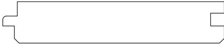
4" BEVELED EDGE PROFILE PLANK DETAIL SCALE 1 : 1
