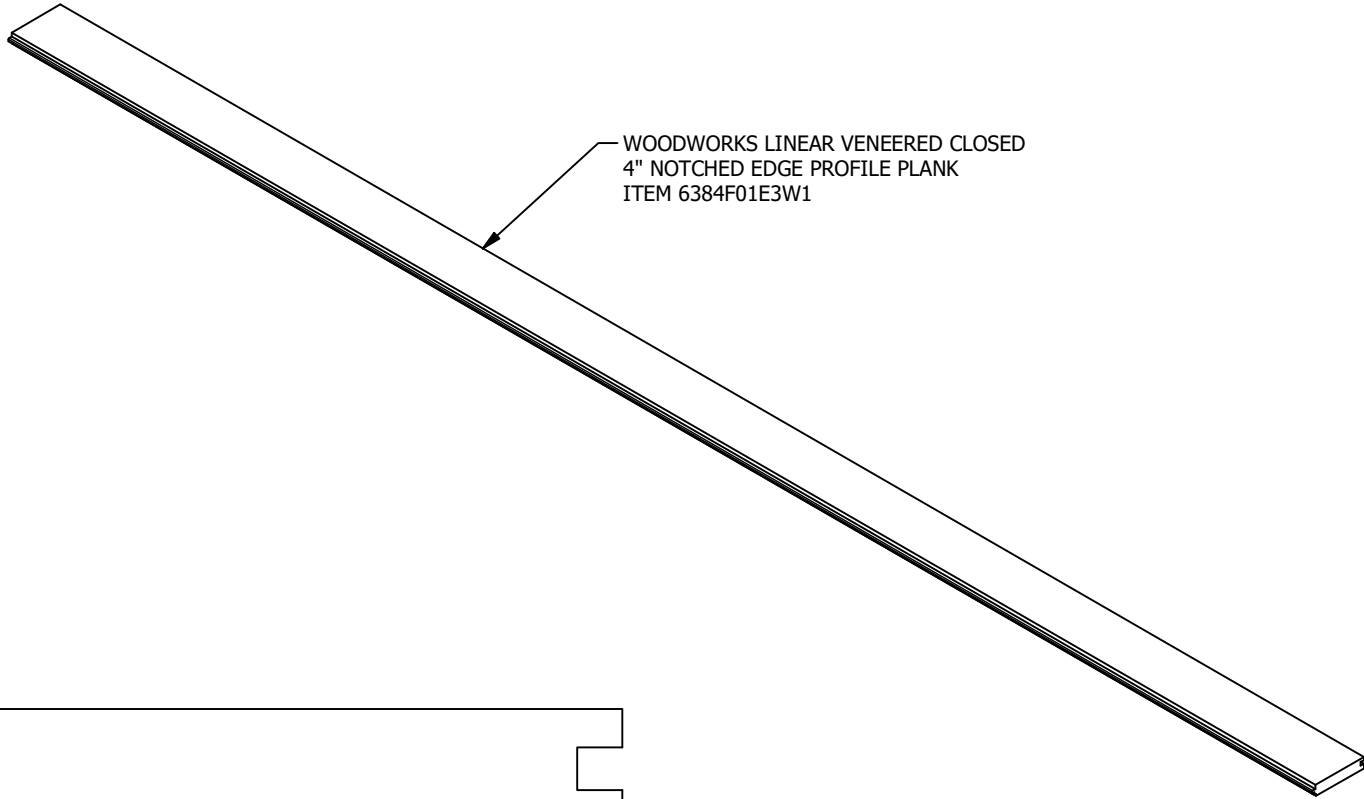
4" NOTCHED EDGE PROFILE PLANK DETAIL SCALE 1 : 1
