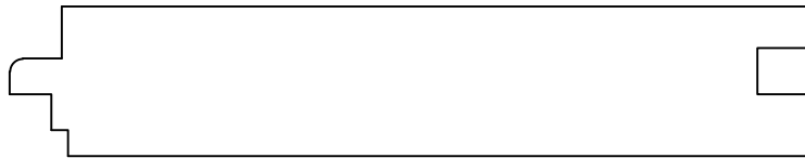
4" NOTCHED EDGE PROFILE PLANK DETAIL SCALE 1 : 1
