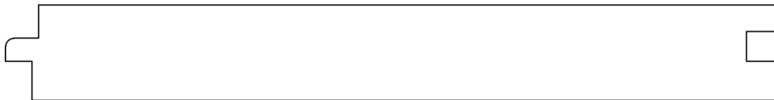
6" SQUARE EDGE PROFILE PLANK DETAIL SCALE 1 : 1
