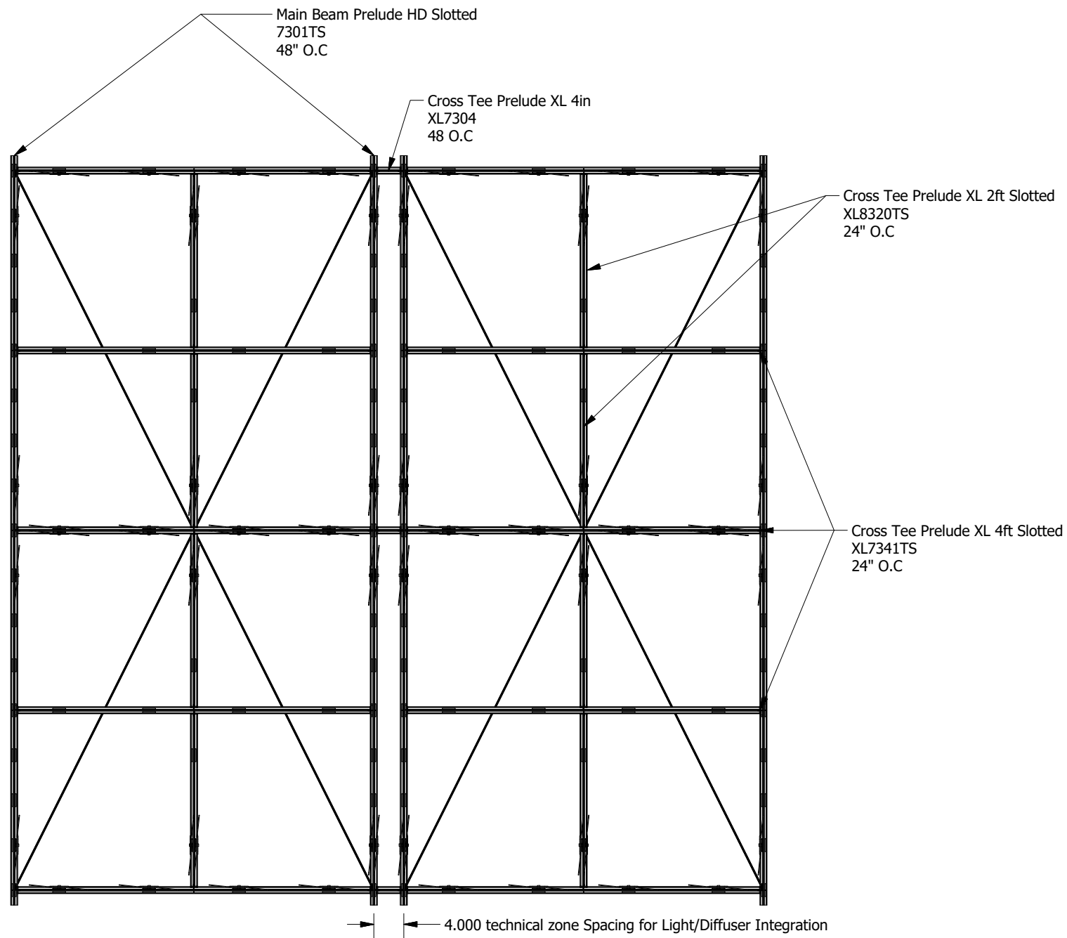
Back of Panel View Scale 1/18
