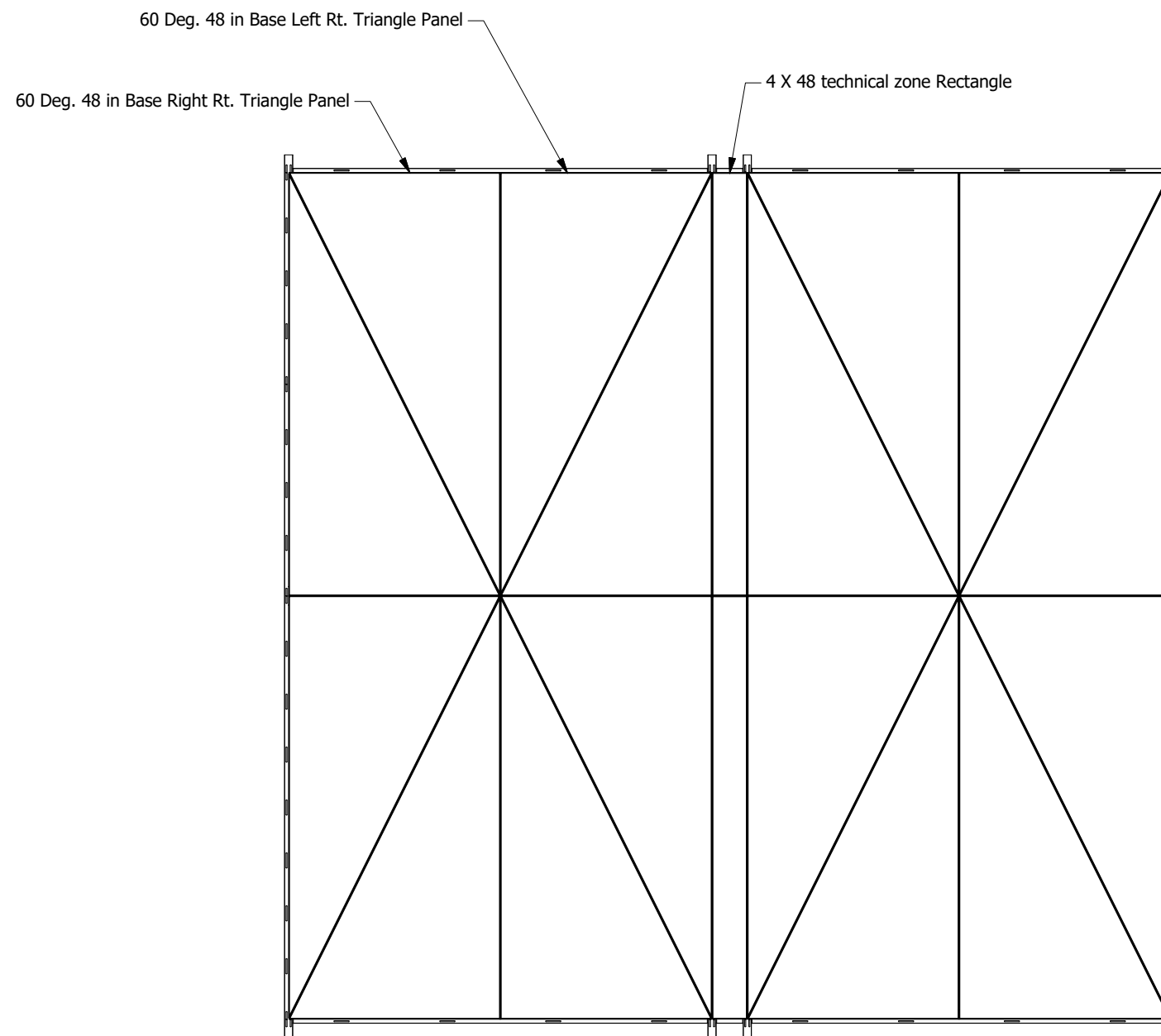
Panel Face View Scale 1/18
