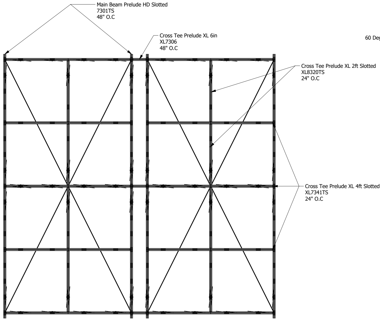
6.000 technical zone Spacing for Light/Diffuser Integration Back of Panel View Scale 1/18
