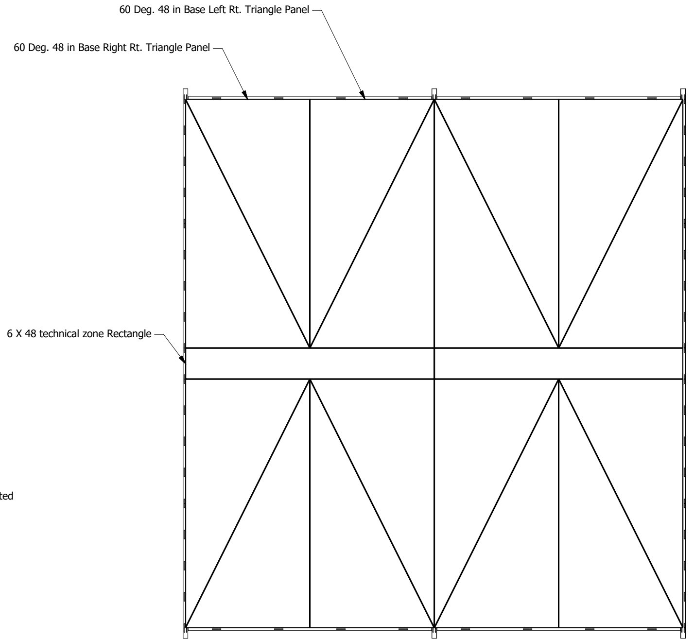
Panel Face View Scale 1/18
