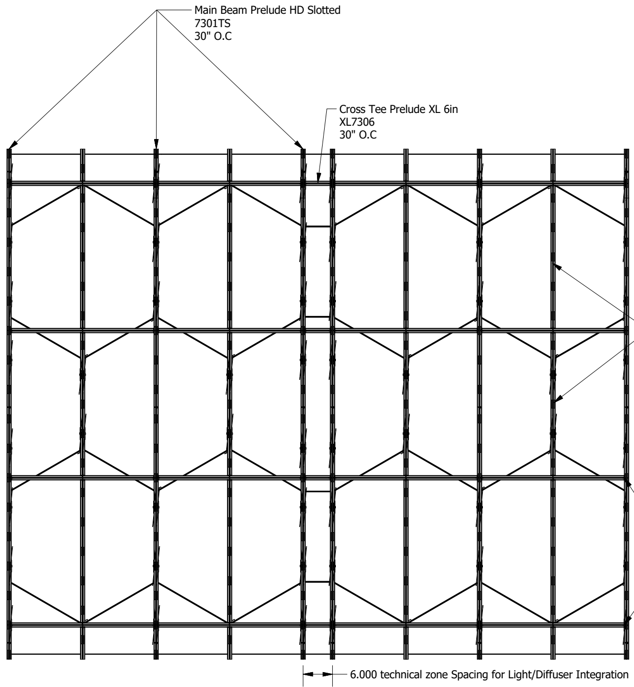
Back of Panel View Scale 1/20
