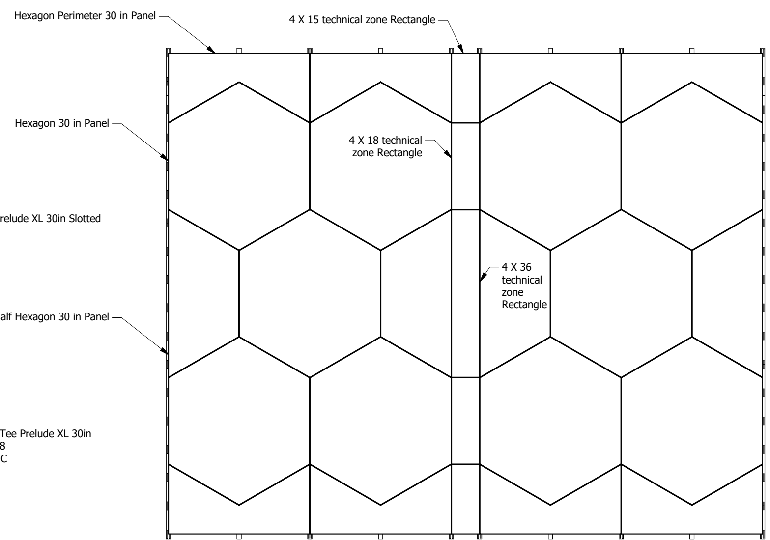
Panel Face View Scale 1/20
