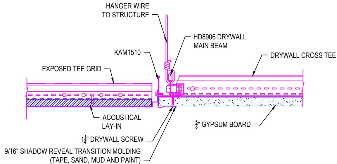
TRADITIONAL FRAMING
