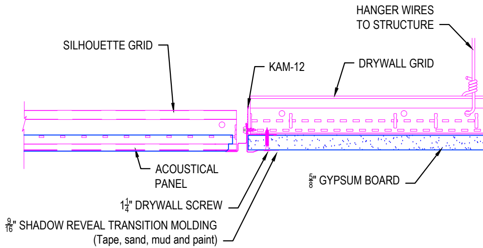
TRADITIONAL FRAMING
