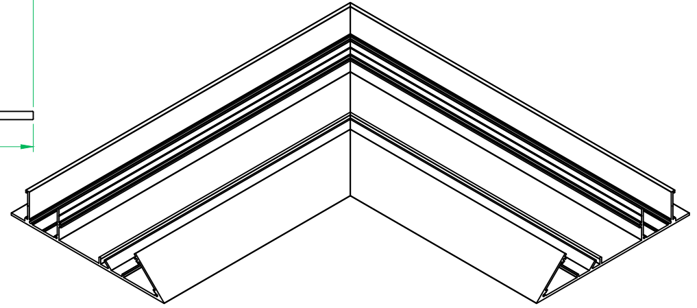
AXIASLCWKEIC CEILING TO WALL INSIDE CORNER
