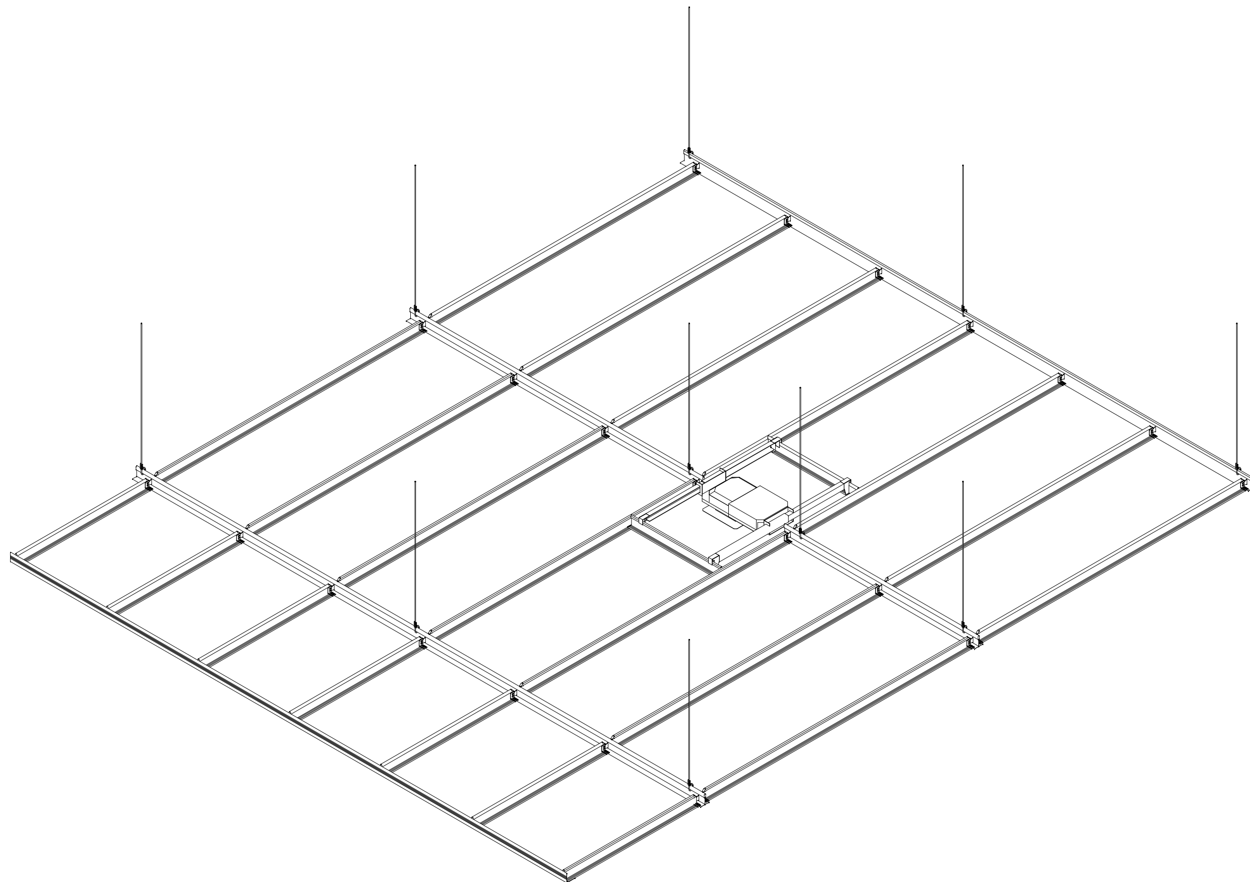
3D VIEW HIGH HAT FIXTURE IN DRYWALL MAIN BEAM CUT
