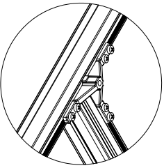
DMTB - Dynamax T Bracket Used to connect main beams and cross-tees to the perimeter extrusion
