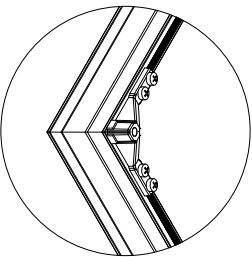
DMILB - Dynamax L Bracket Used to connect perimeter extrusion corners together.
