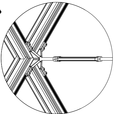
Turnbuckles and threaded rods are used to connect to X-brackets to create a structural support for the grid
