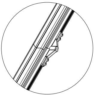
DMIB - Dynamax I Bracket Used to splice together main beams ends
