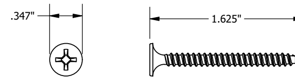
8187L16 #6 x 1-5/8" Painted Head Sharp Point Screw for Screw Installation to Wall
