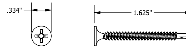
8188L16 #6 x 1-5/8" Painted Head Drill Point Screw for Screw Installation to Wall
