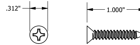
6527 #8 x 1" Screw for Magnet Installation
