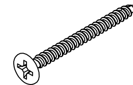
8187L16 #6 x 1-5/8" Painted Head Sharp Point Screw for Screw Installation to Wall
