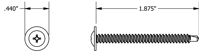
6489 #8 x 1-7/8" Screw for Washer Installation
