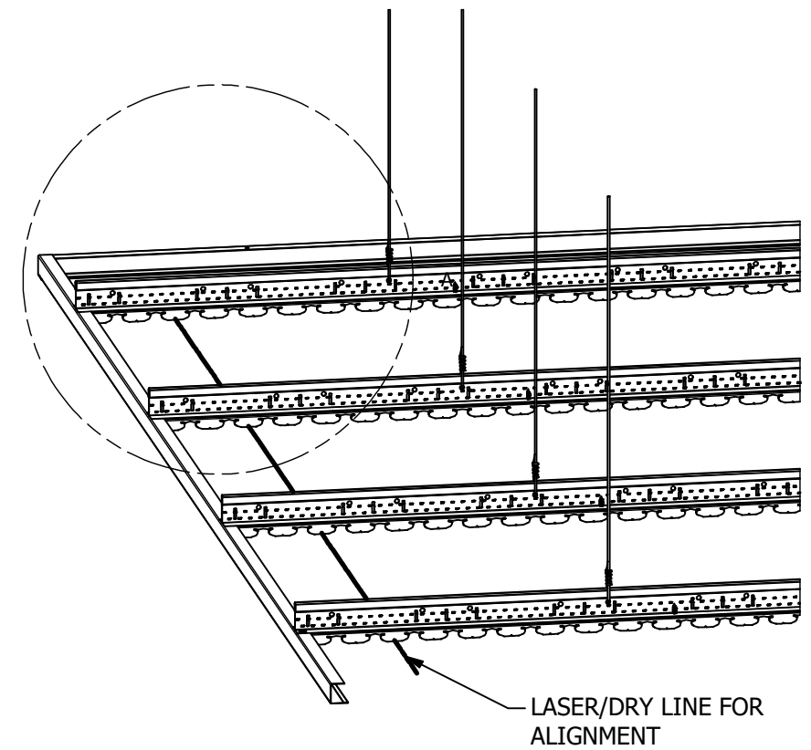
CARRIER ALIGNMENT ISO VIEW SCALE 1 / 10
