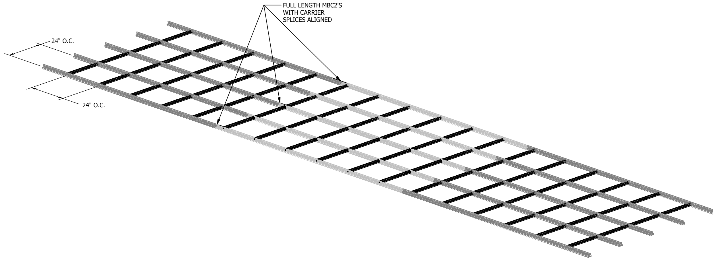
STANDARD GRID LAYOUT ALIGNED MBC2
