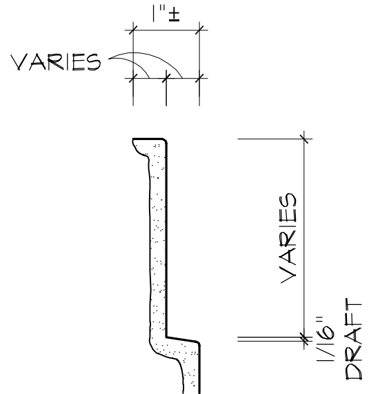
TOP SECTION
