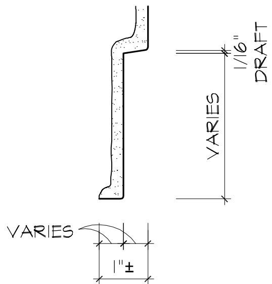
BOTTOM SECTION
