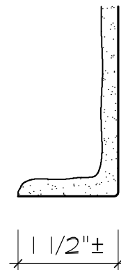
BOTTOM SECTION
