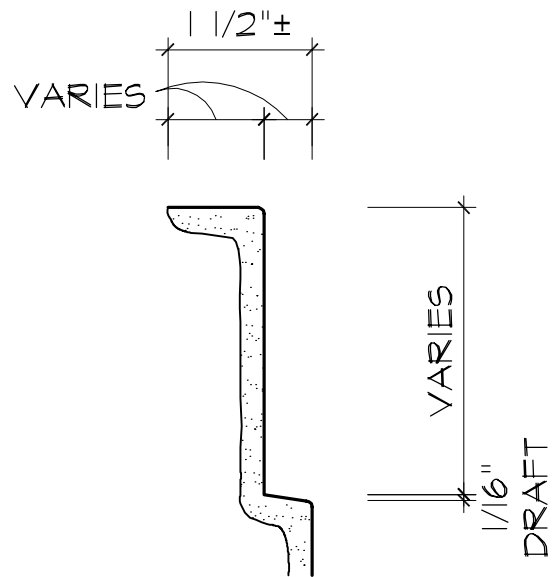
TOP SECTION
