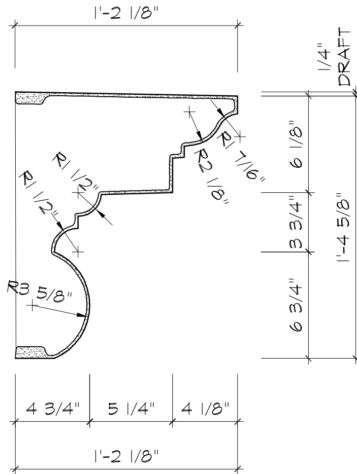
SECTION
