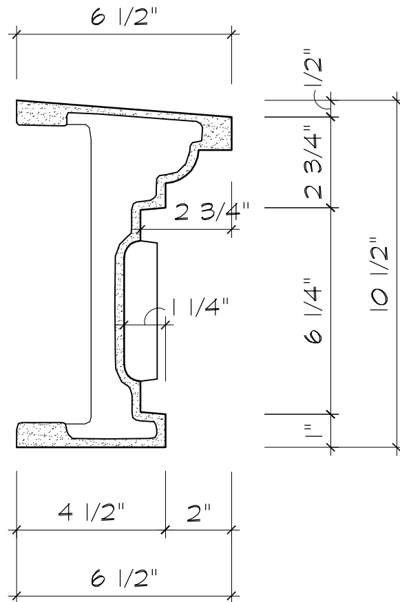
SECTION
