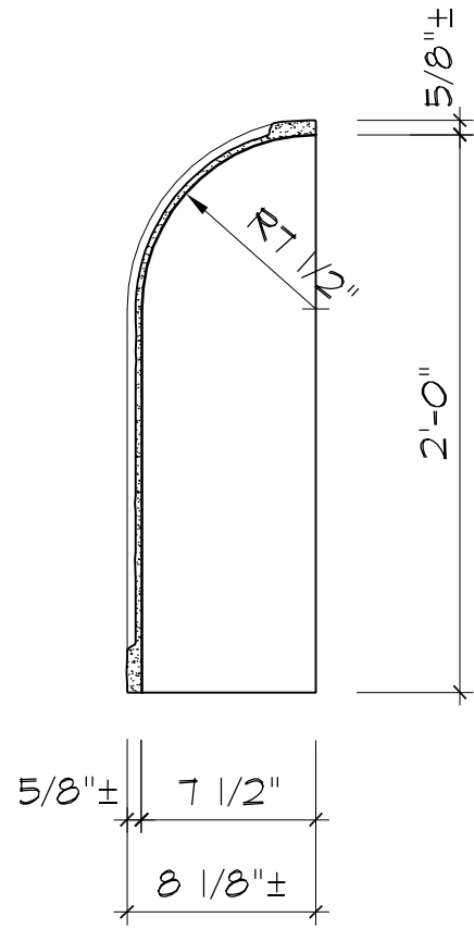
SECTION
