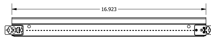
BPM757524 Suprafine 75° Cross Tee - 24" MBS SCALE 1 / 4
