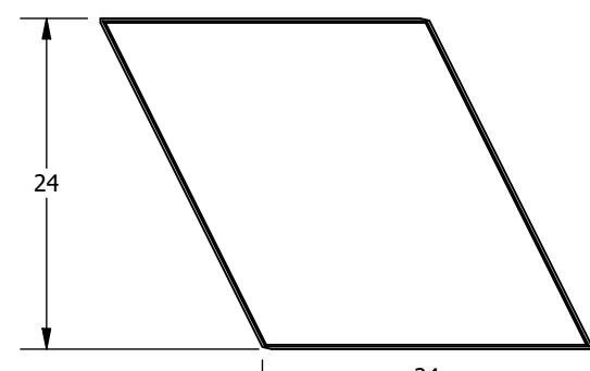
Ultima 9/16" Beveled Tegular - 60 Deg. 24 in Base Left Parallelogram 100314
