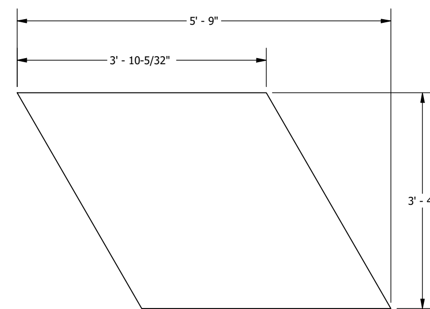
BP7101F02P01-??? PAINTED SS SHAPES 60 DEG PARALLELOGRAM SCALE 1 : 18
