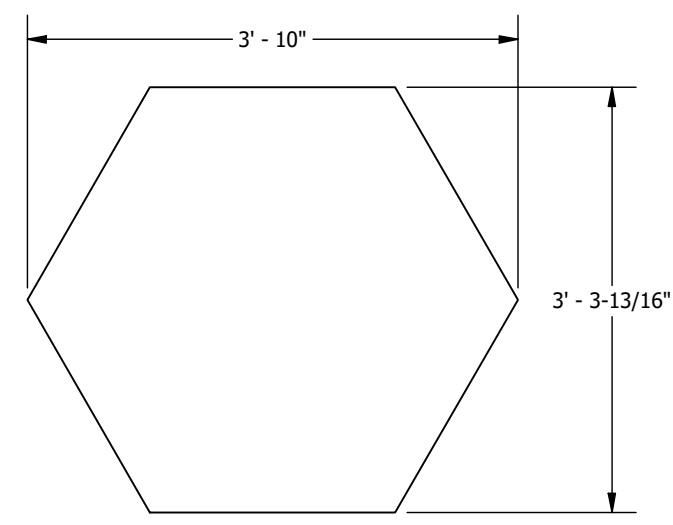
BP5444F02G01-??? PAINTED SS SHAPES HEXAGON 4FT x 4FT SCALE 1 : 18
