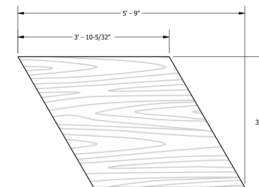
BP7101F04P01-??? WOOD LOOK SS SHAPES 60 DEG PARALLELOGRAM SCALE 1 : 18
