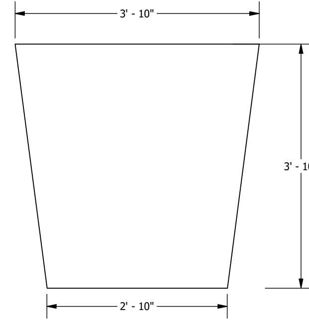
BP5445F02Z02-??? PAINTED SS SHAPES TRAPEZOID 4FT x 4FT SCALE 1 : 18
