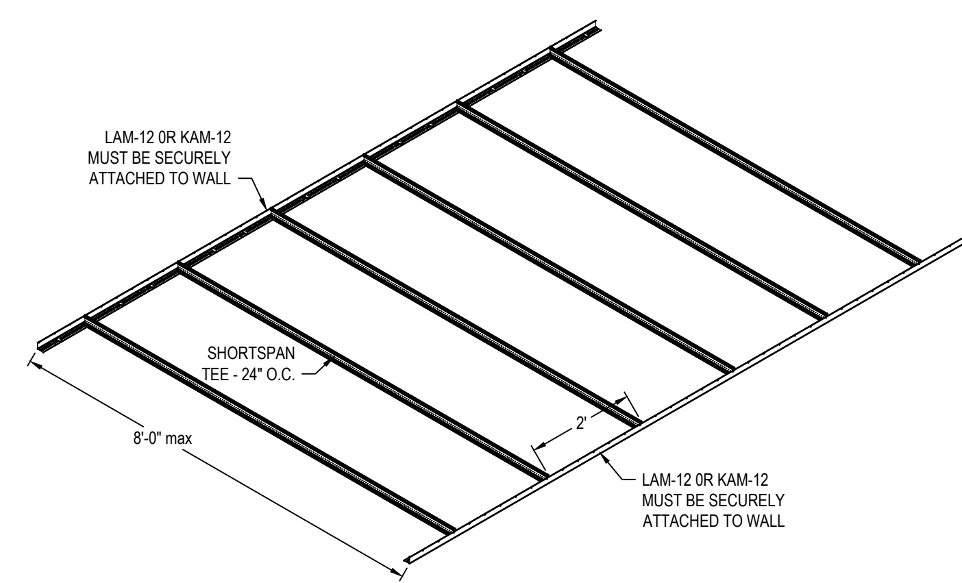
8 SHORTSPAN LAYOUT WITH 8'-0" SPAN
