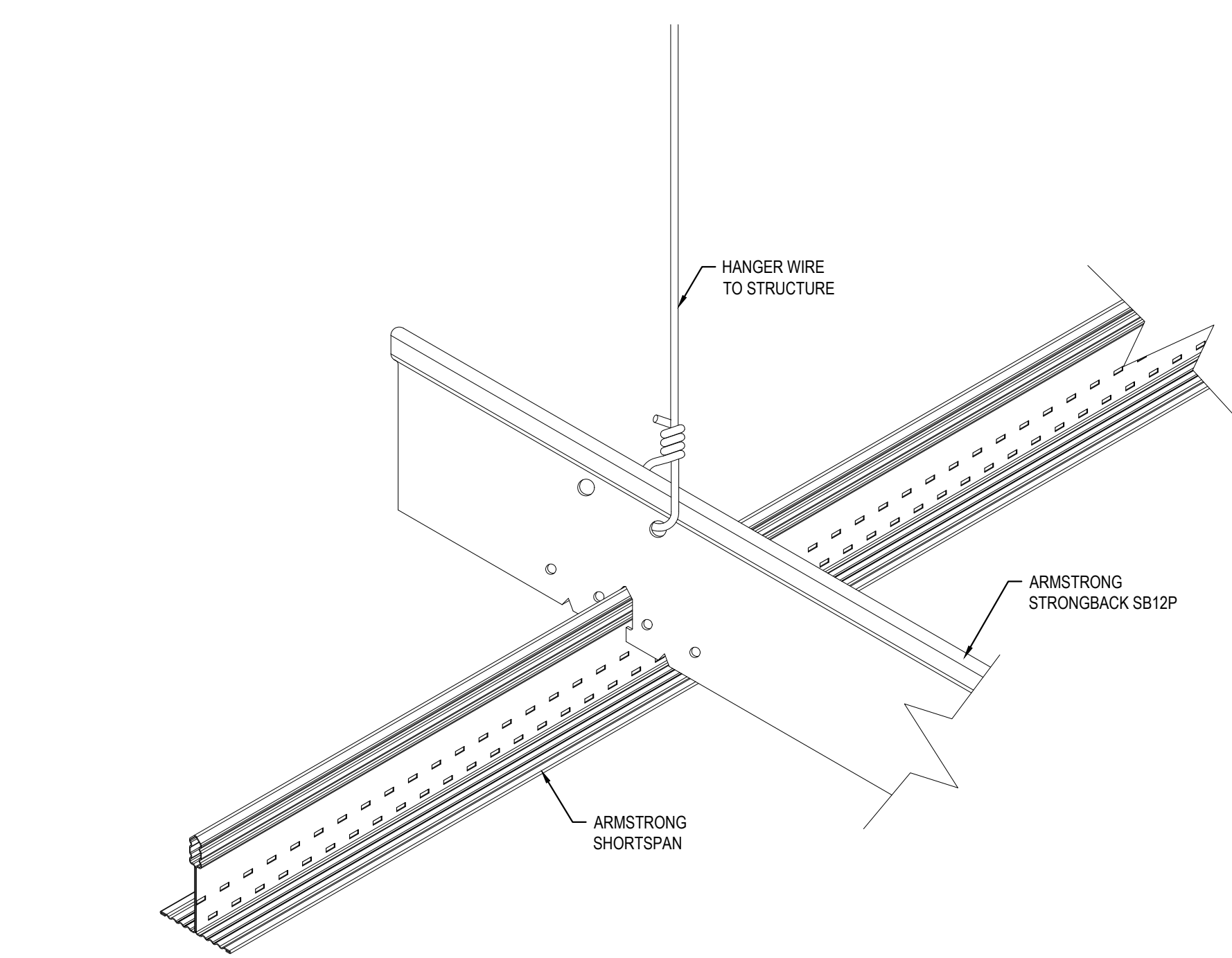
6 SHORTSPAN WITH STRONGBACK APPLICATION
