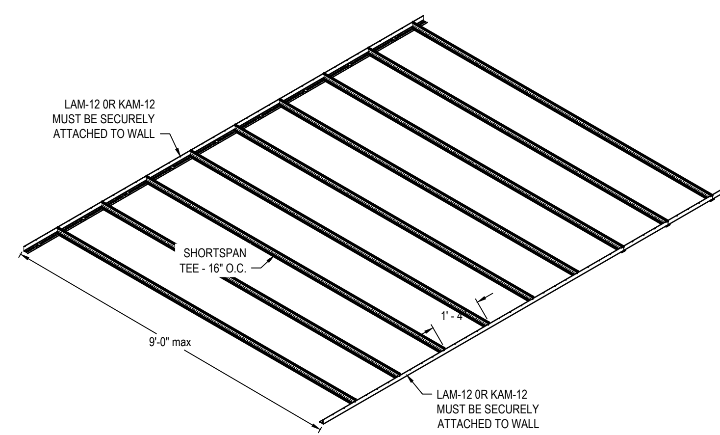
7 SHORTSPAN LAYOUT WITH 9'-0" SPAN
