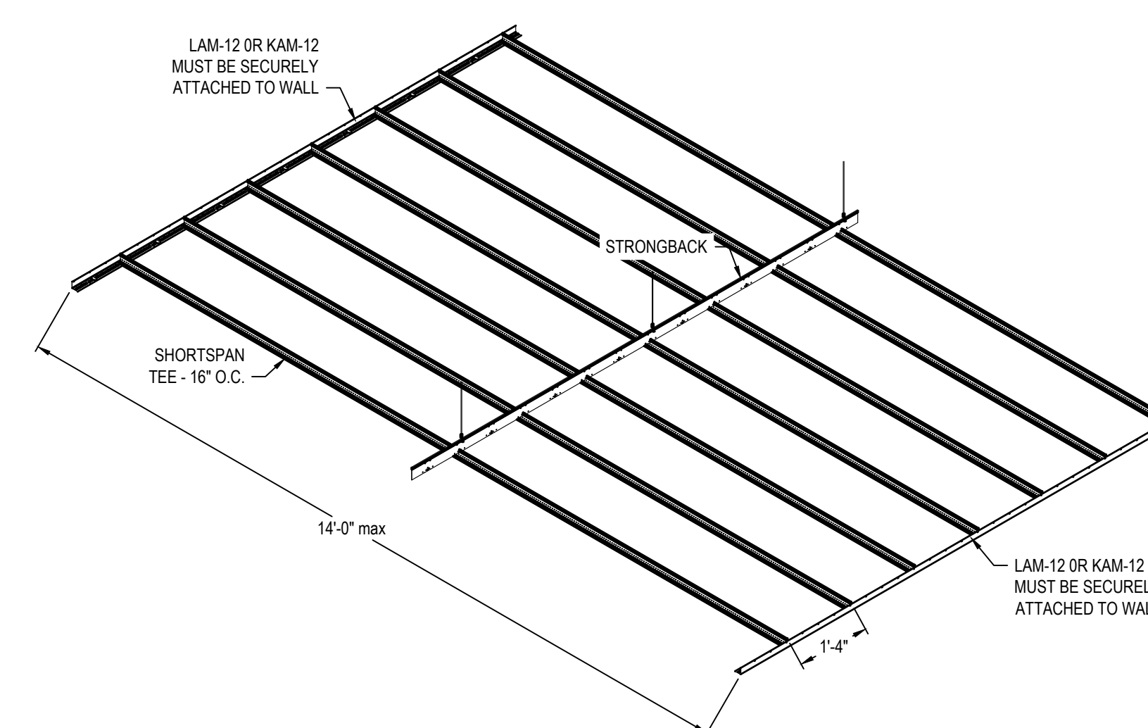
9 SHORTSPAN LAYOUT WITH 14' SPAN 16" O.C.
