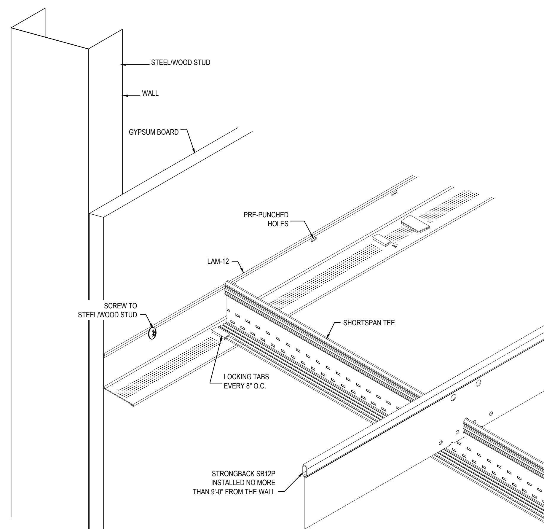
4 SHORTSPAN AT WALL
