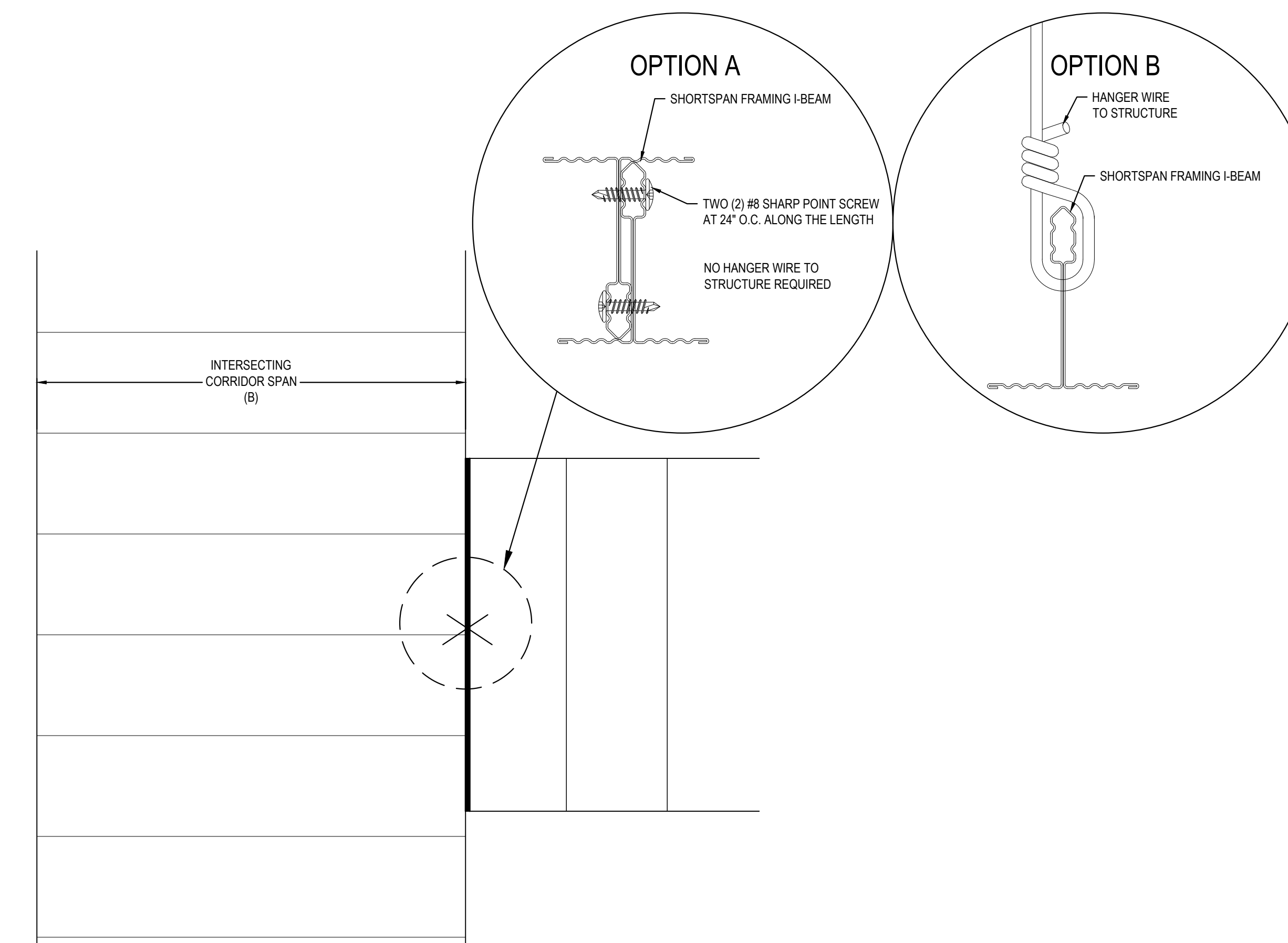
5 SHORTSPAN INTERSECTION CORRIDORS WITH I-BEAM GIRDER
