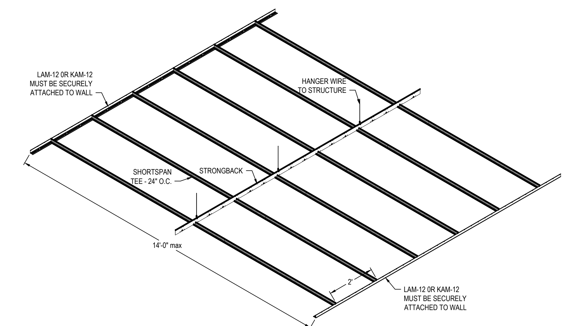
10 SHORTSPAN LAYOUT WITH 14' SPAN 24" O.C.
