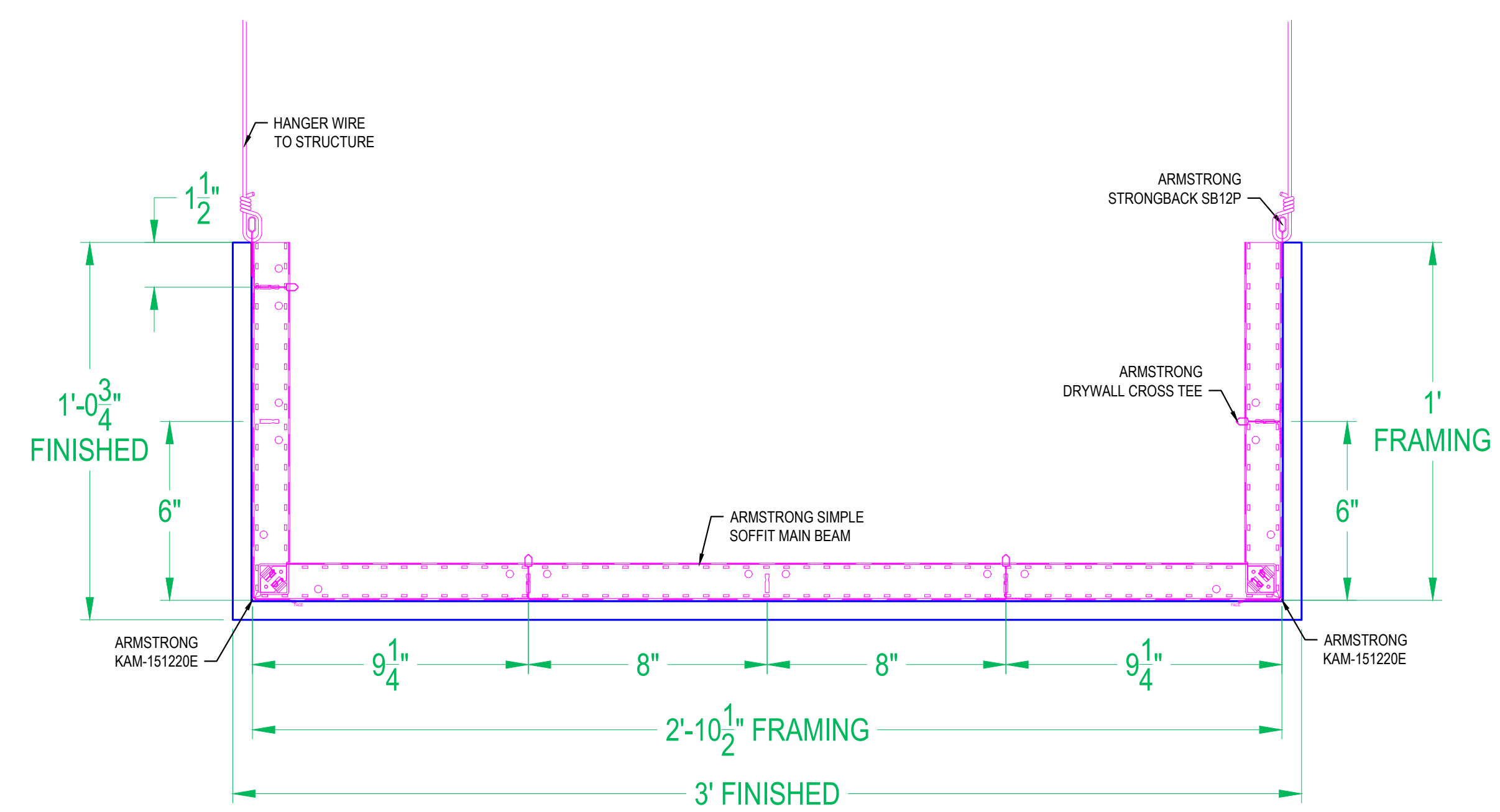
22 SIMPLE SOFFIT SSU123612
