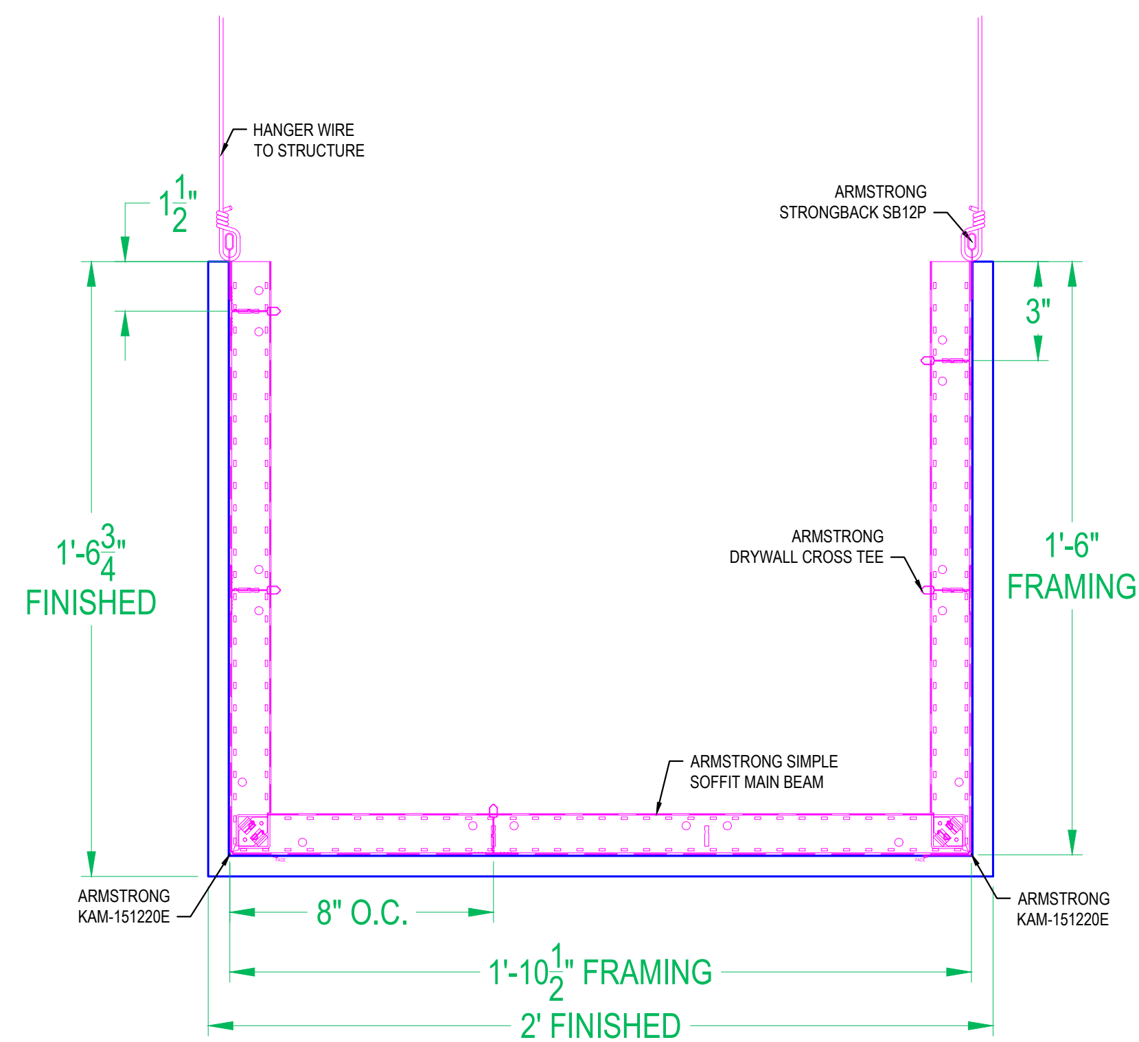
21 SIMPLE SOFFIT SSU182418
