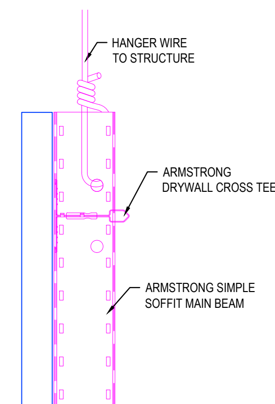
14 SIMPLE SOFFIT WITH HANGER WIRE
