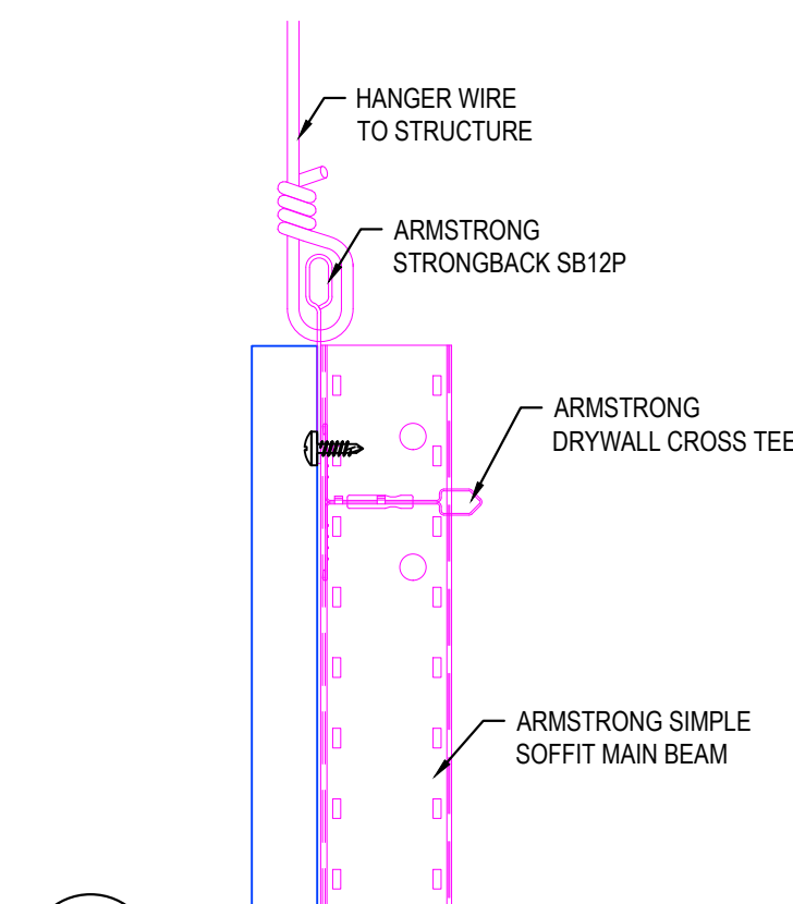
13 SIMPLE SOFFIT WITH STRONGBACK SUPPORT
