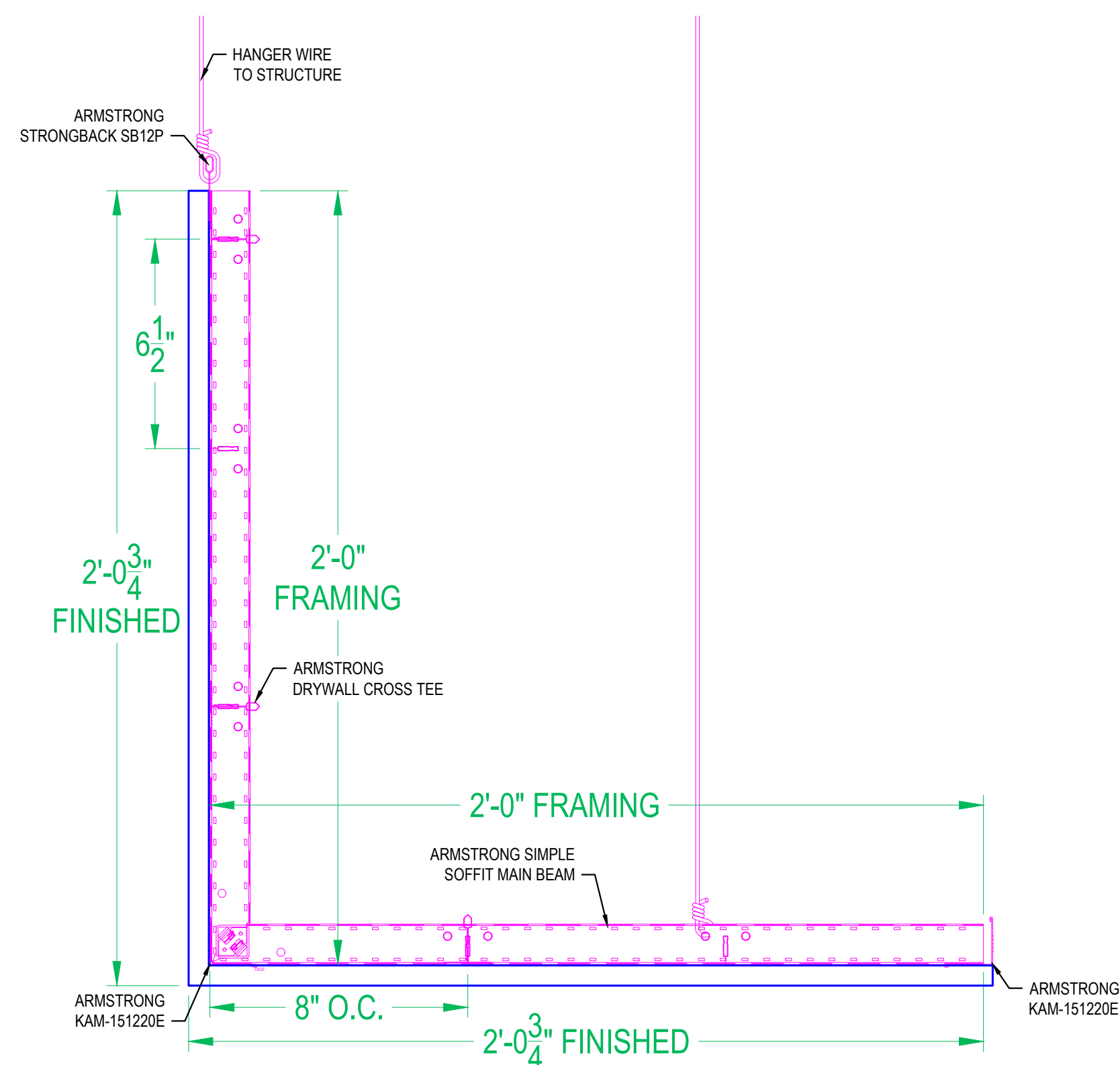
15 SIMPLE SOFFIT SSLU3636
