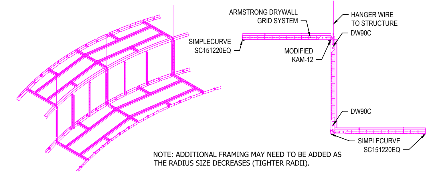
16 DRYWALL STEP SOFFIT SOFFIT WITH SIMPLECURVE
