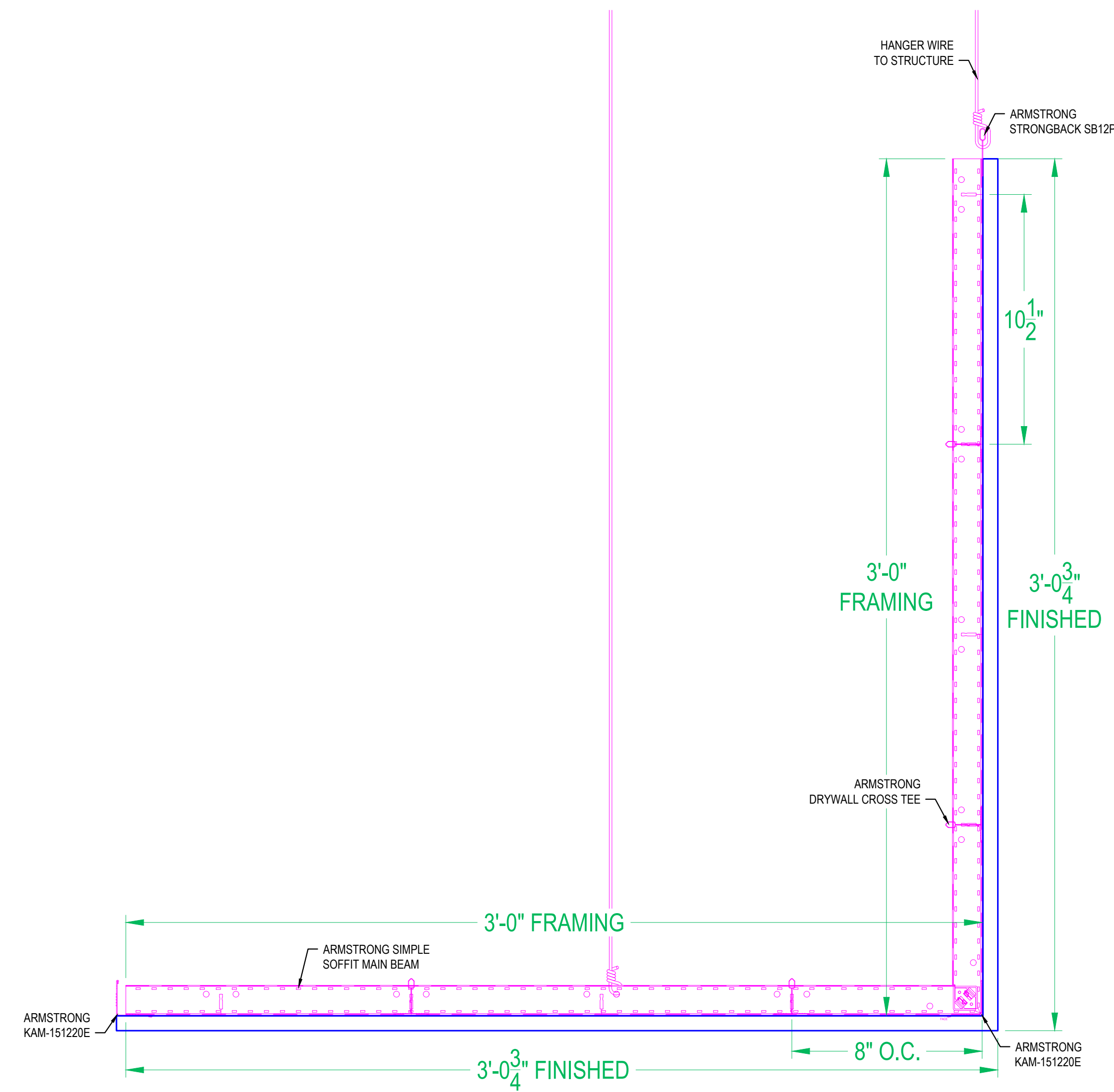
15 SIMPLE SOFFIT SSLU3636
