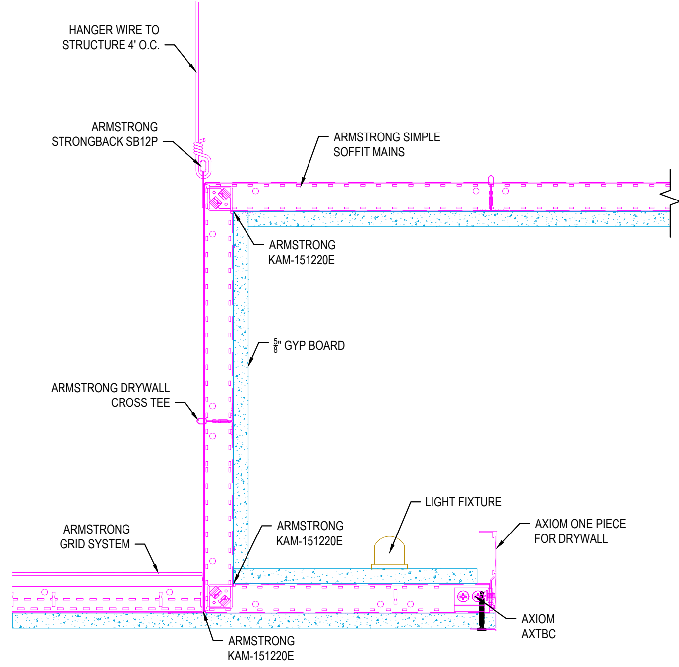
6 SIMPLE SOFFIT LIGHT COVE WITH AXIOM ONE PIECE
