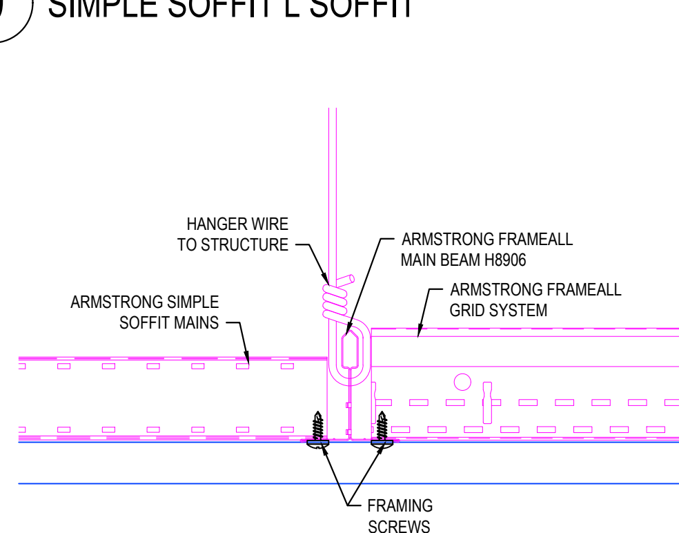
12 SIMPLE SOFFIT FLUSH TRANSITION TO FRAMEALL DRYWALL GRID
