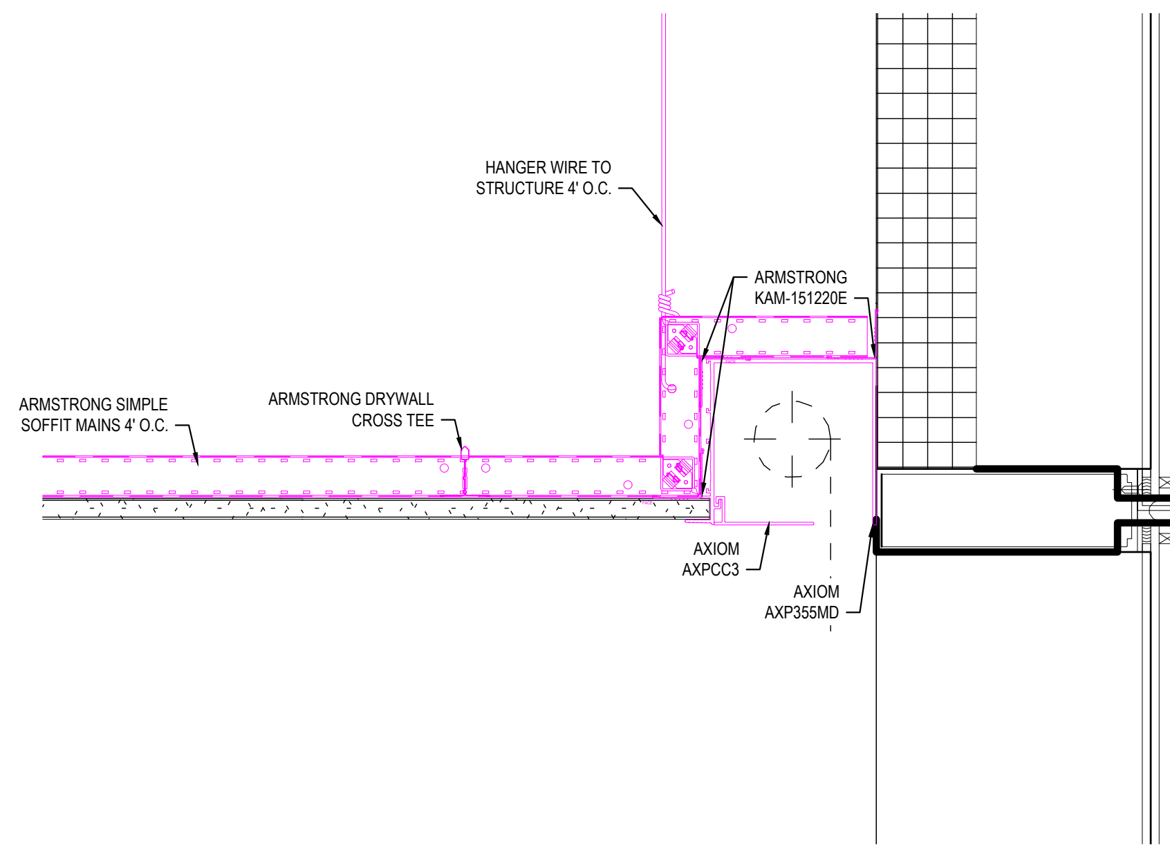
7 SIMPLE SOFFIT SOFFIT AROUND AXIOM BUILDING PERIMETER POCKET
