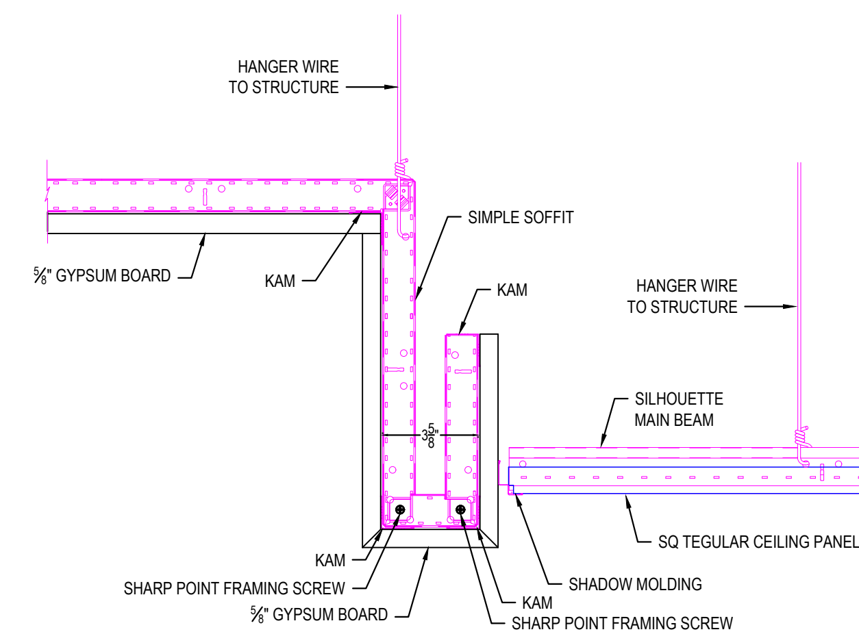
15 SIMPLE SOFFIT 3-5/8" BULKHEAD
