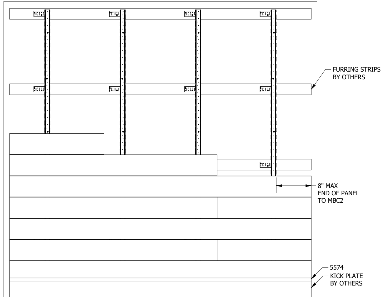
FRONT VIEW SCALE 1 / 18
