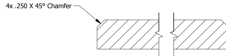
SECTION A-A SCALE 1 / 2
