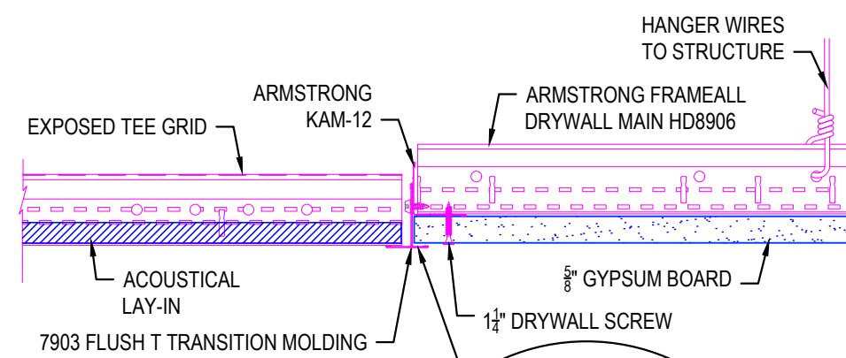
4 7903 TRANSITION MOLDING
