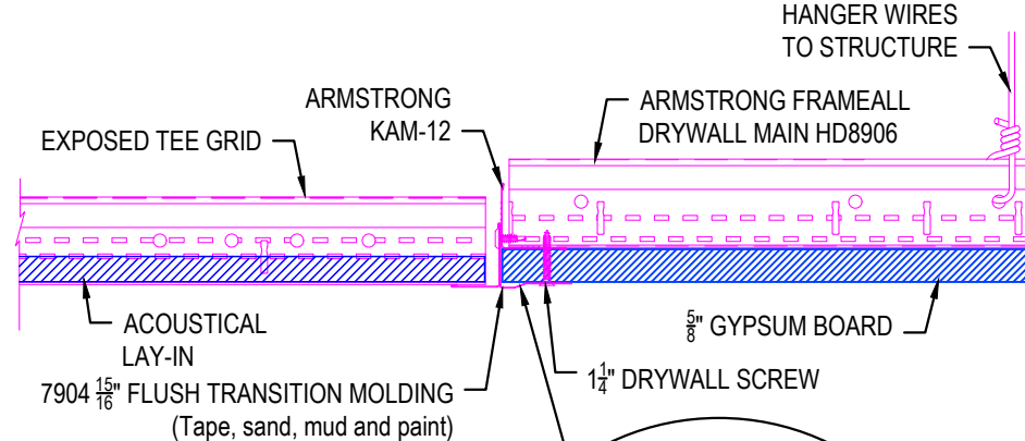
5 7904 TRANSITION MOLDING
