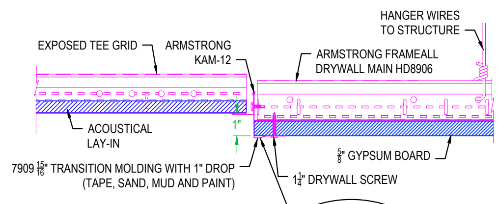
9 7909 TRANSITION MOLDING
