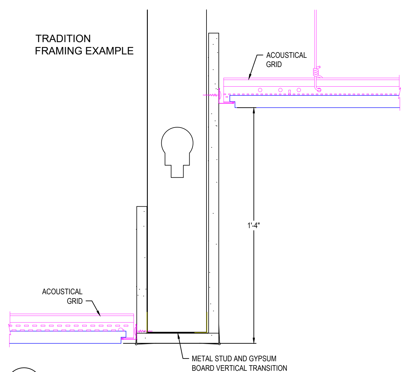
16 STUD DROP TRANSITION COMPARISON
