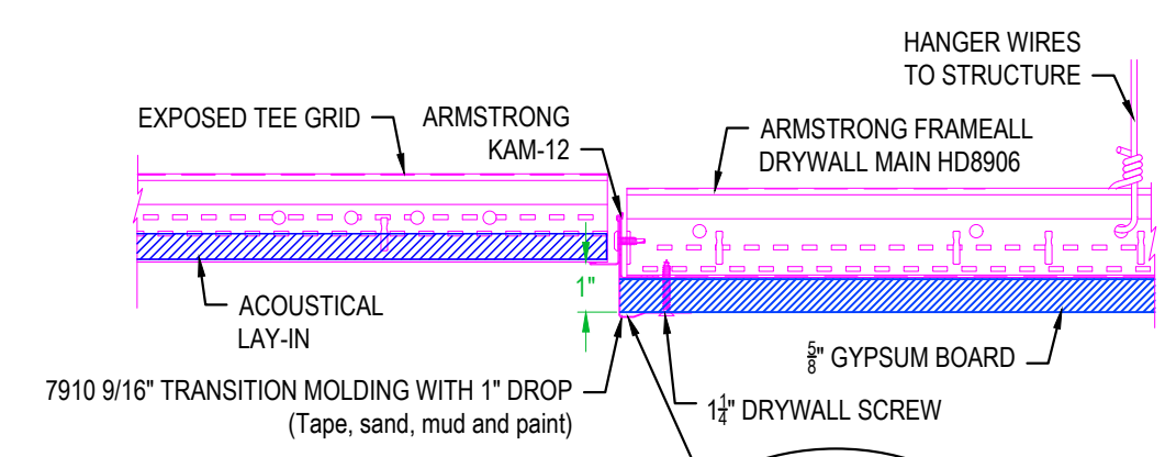
10 7910 TRANSITION MOLDING
