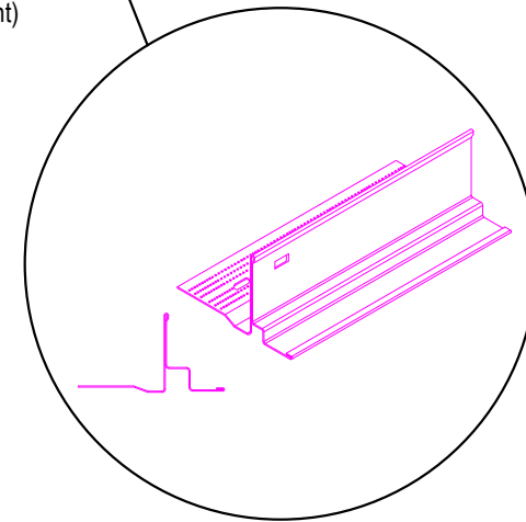
2 7901 TRANSITION MOLDING
