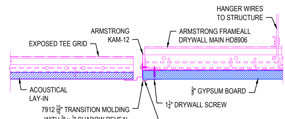
12 7912 TRANSITION MOLDING
