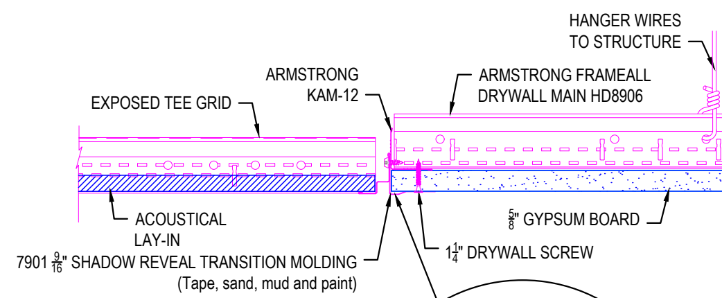
2 7901 TRANSITION MOLDING
