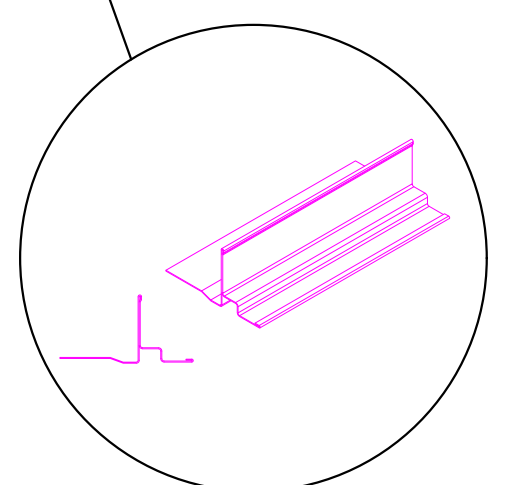
11 7911 TRANSITION MOLDING
