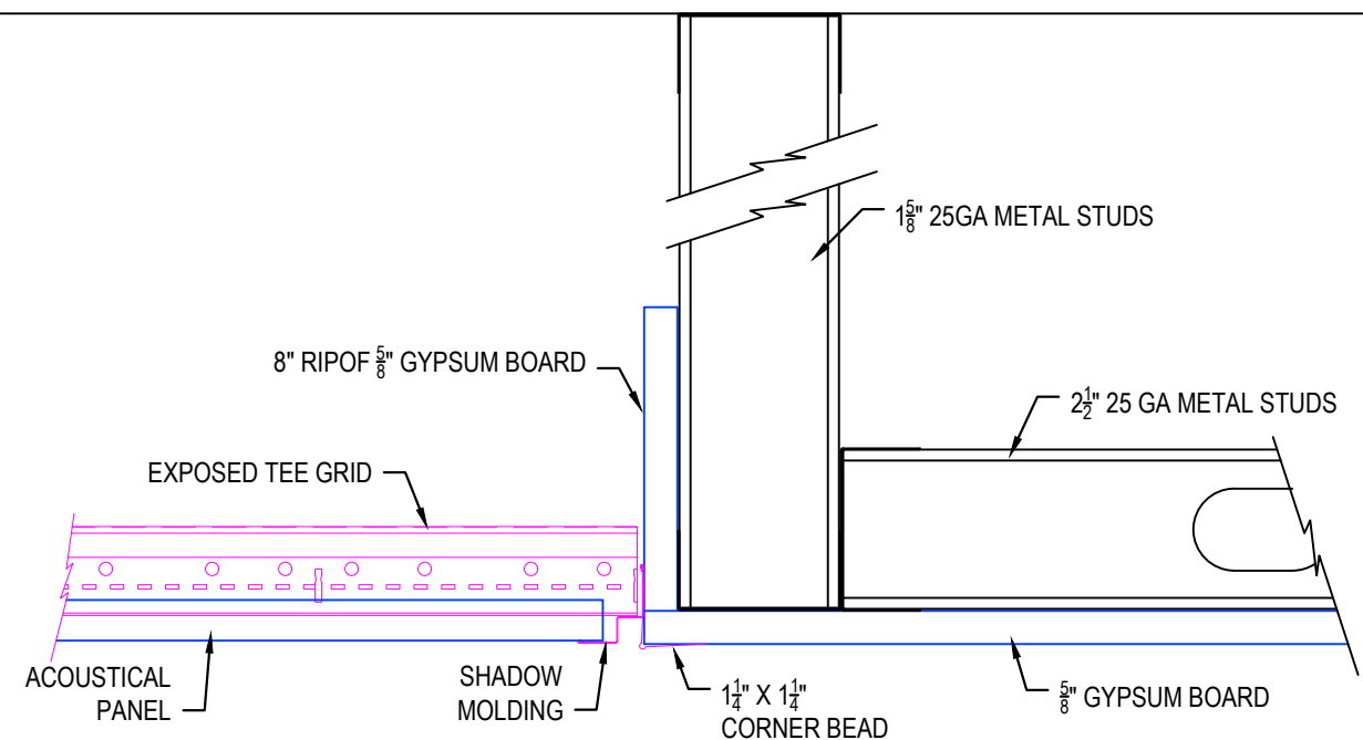
1 TRADITION FRAMING COMPARISON
