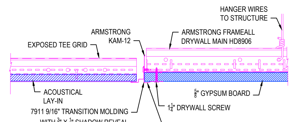
11 7911 TRANSITION MOLDING
