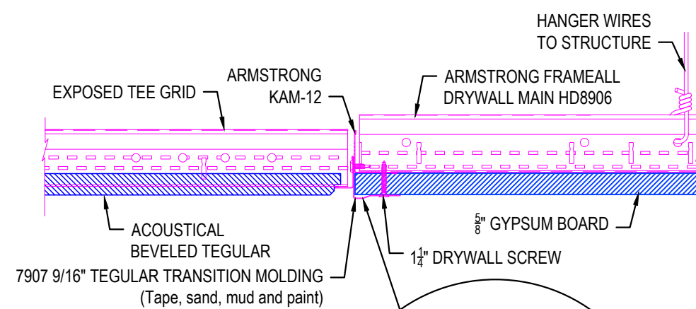
7 7907 TRANSITION MOLDING
