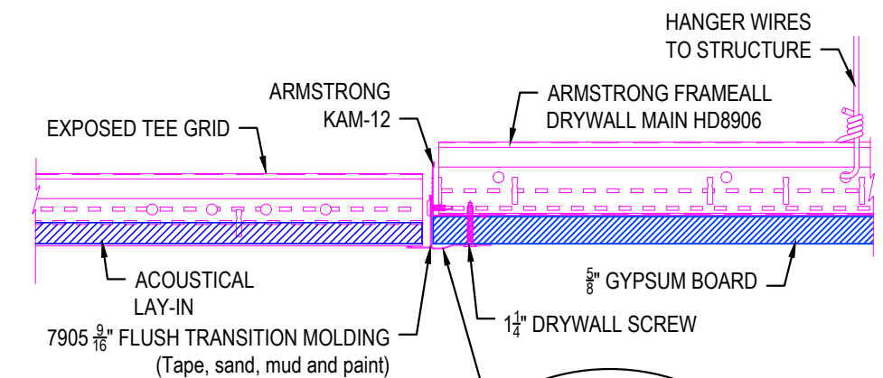
6 7905 TRANSITION MOLDING
