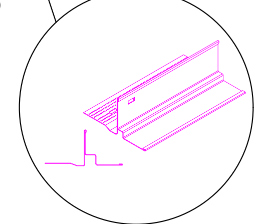
3 7902 TRANSITION MOLDING
