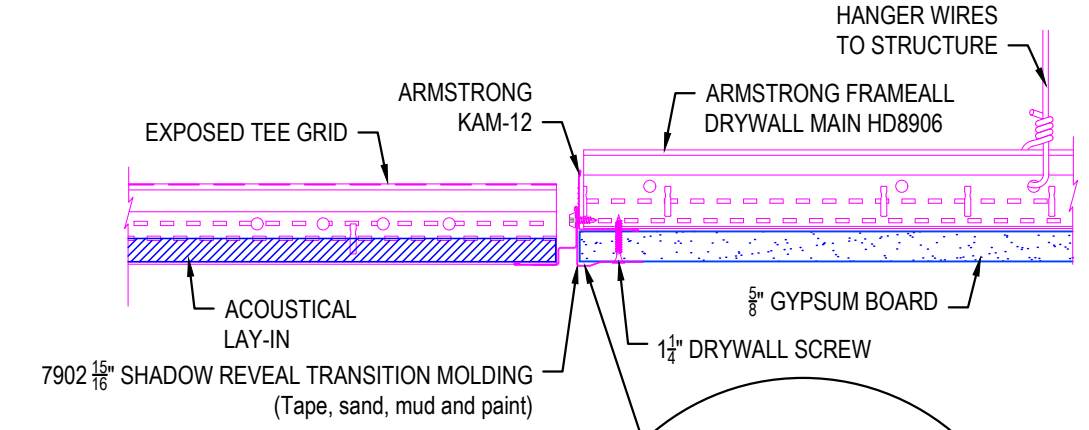
3 7902 TRANSITION MOLDING
