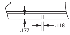
DETAIL A SCALE 1 / 2
