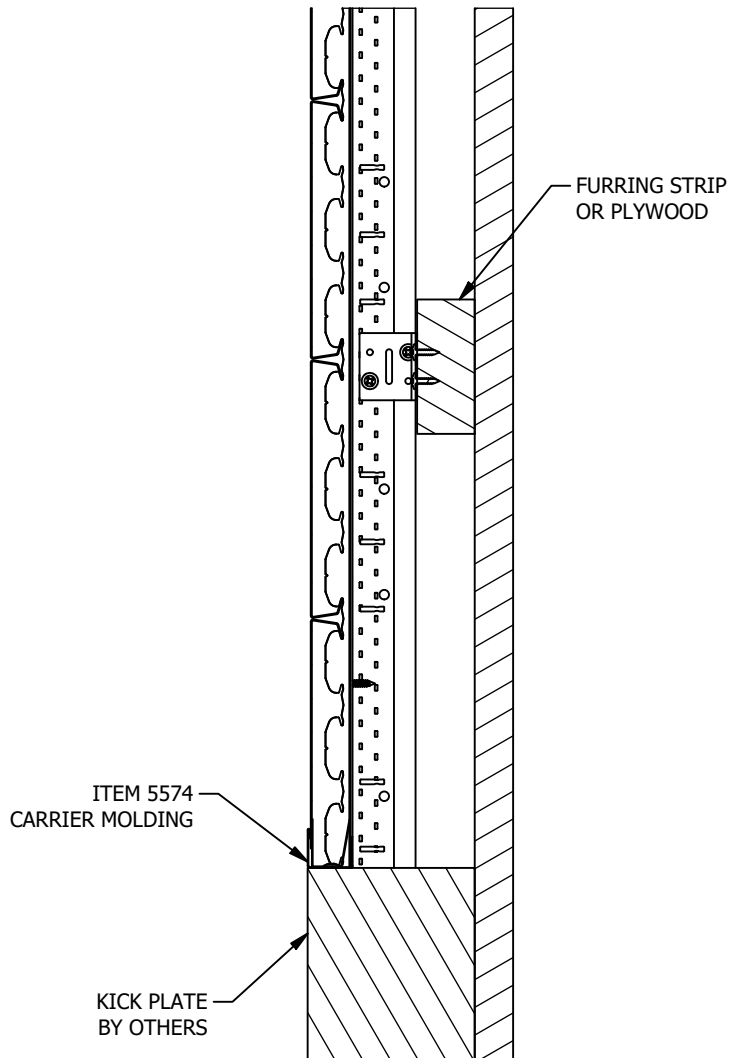
SECTION SIDE VIEW OF SYNCHRO WALL INSTALLATION SCALE 1 / 5
