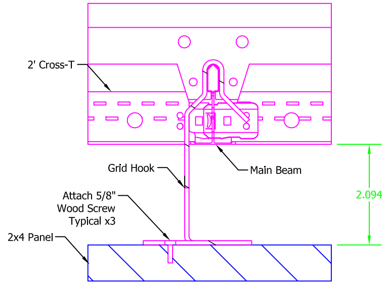
DETAIL B SCALE 1 / 2
