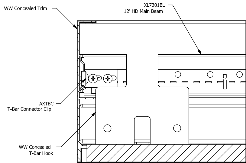
SECTION C-C SCALE 1 / 2
